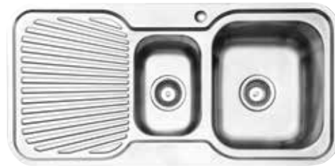
1 & 1/4 Bowl – 22 litres & 9 litres + drainer IS9LS3 (Left hand bowl) IS9RS3 (Right hand bowl) – pictured 600 cabinet – L 980mm x B 480mm x D 180mm
