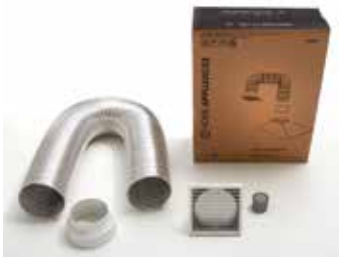
DKE Eave Duct Kit Universal kit – suits 125mm & 150mm.
